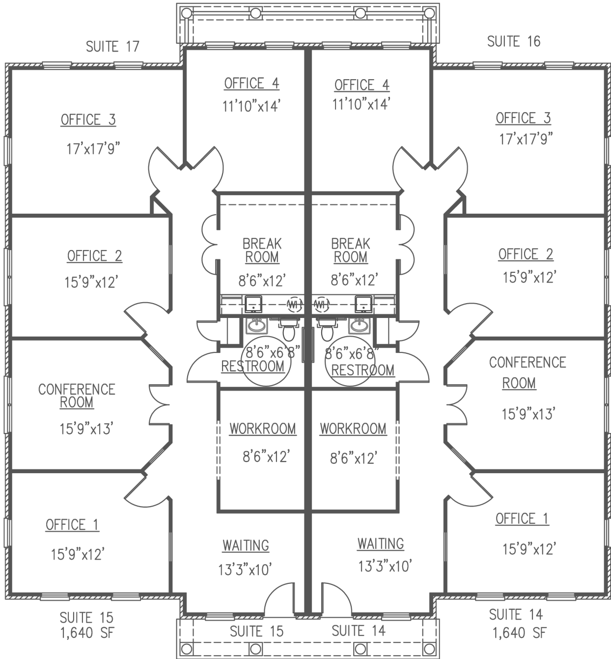
ONE-STORY ELEVATION 3,280 SF
